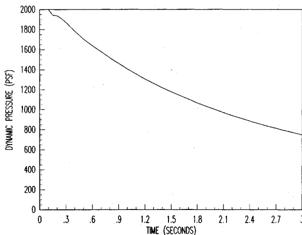
e) Dynamic pressure vs time
