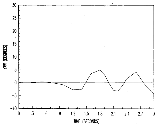
c) Yaw vs time
