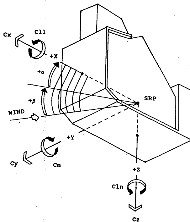
Fig. 5 SHABP input geometry model with aerocoefficients.
