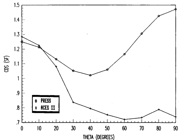
Fig. 8 Drag comparison of PRESS and ACES II.
